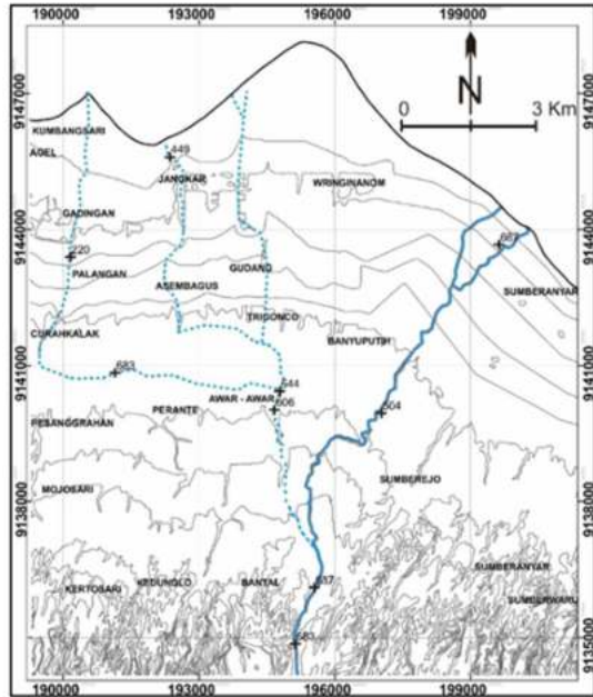
Fig. 15 Distribution of \text{SO}_4 measurements of water samples (+: \text{SO}_4 concentration in ppm).
