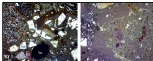
Fig. 9 Shows micrograph of basalt (ba) fragments, lithic (pumice breccia: pb), plagioclase (plg), pyroxene (px), and hematite (he) from the lahar breccia unit of Bogor Formation. Hematite is formed due to rocks interacting with the acidic water of the Banyupait River (location at Sukorejo).
