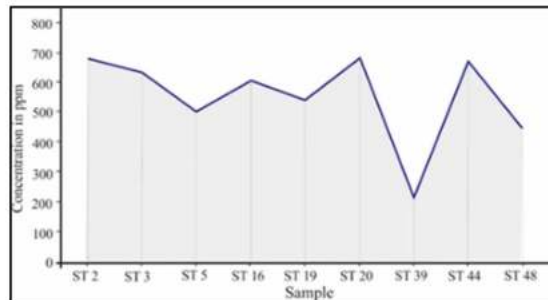
Fig. 16 Distribution of \text{SO}_4 measurements of water samples (in ppm).
