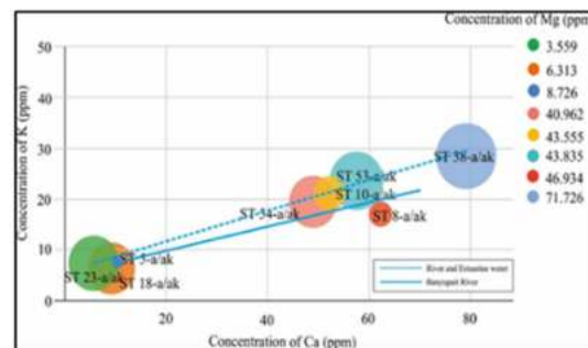
Fig. 25 The Ca-K-Mg elements' balloon diagram shows that the Ca, K, and Mg show a linear pattern.
